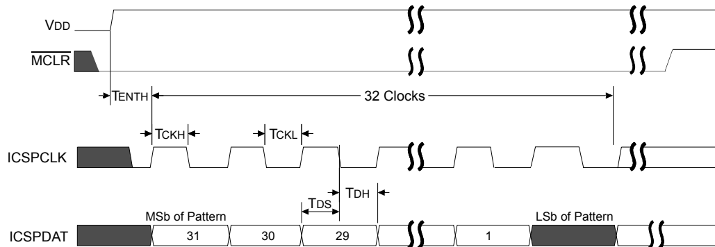
Figure 2-4. LVP Entry (Powered)
