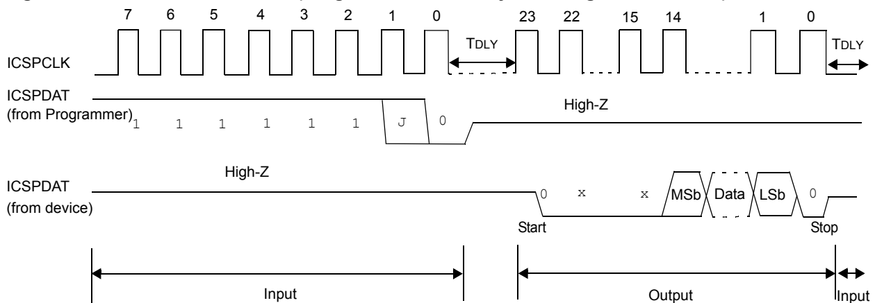
Figure 2-9. Read Data from NVM (EEPROM)
